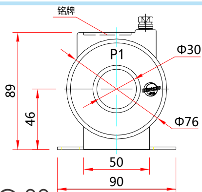
LMZ1-0.66G-30
